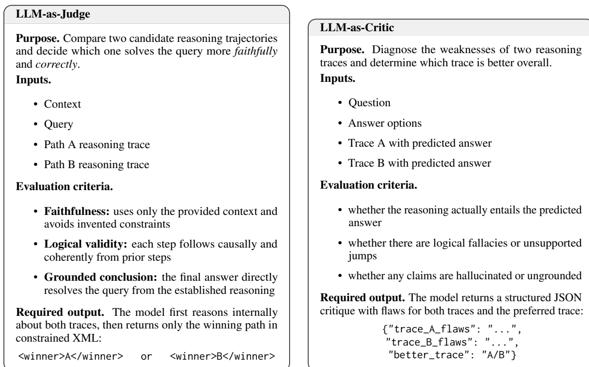
Figure 2: LLM-based routing prompts. The judge prompt is verdict-oriented: it compares two reasoning paths under faithfulness and logical soundness criteria and outputs only the winner. The critic prompt is diagnosis-oriented: it identifies flaws in each trace before selecting the better one in structured JSON form.
